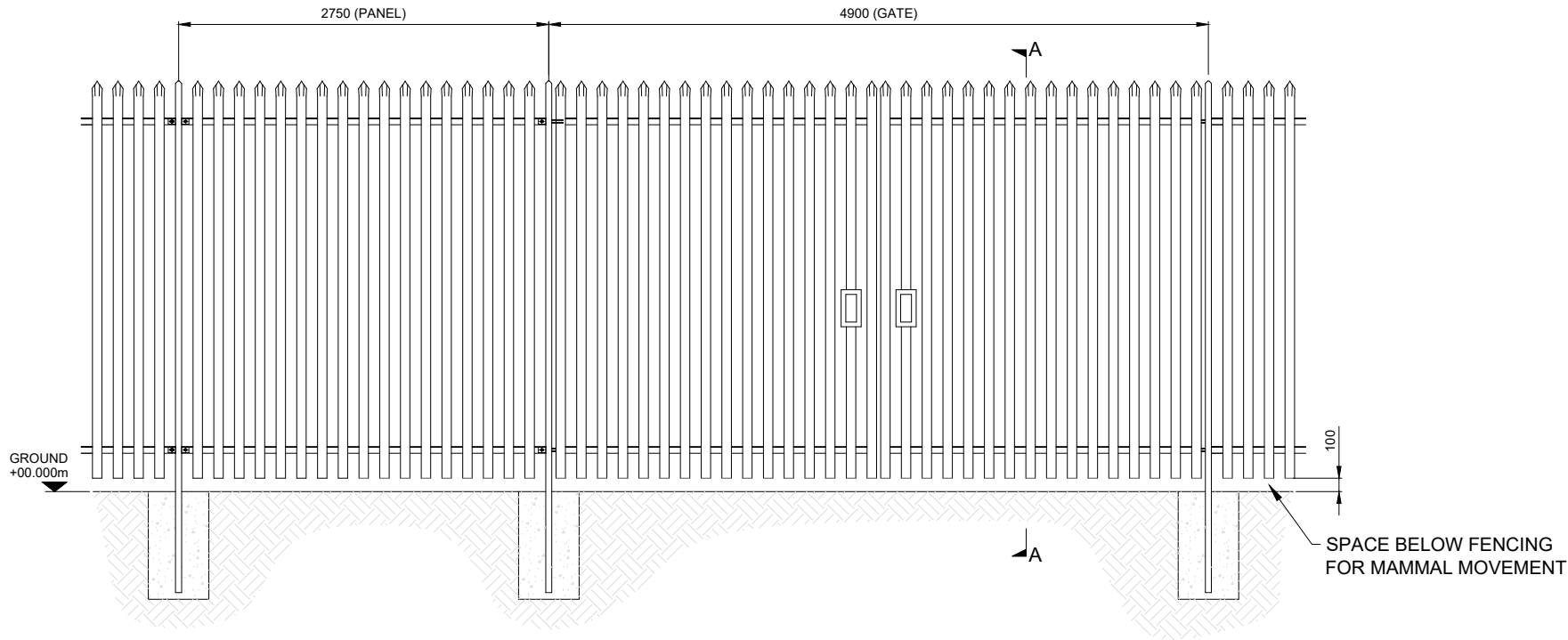
PALISADE FENCE DETAIL
