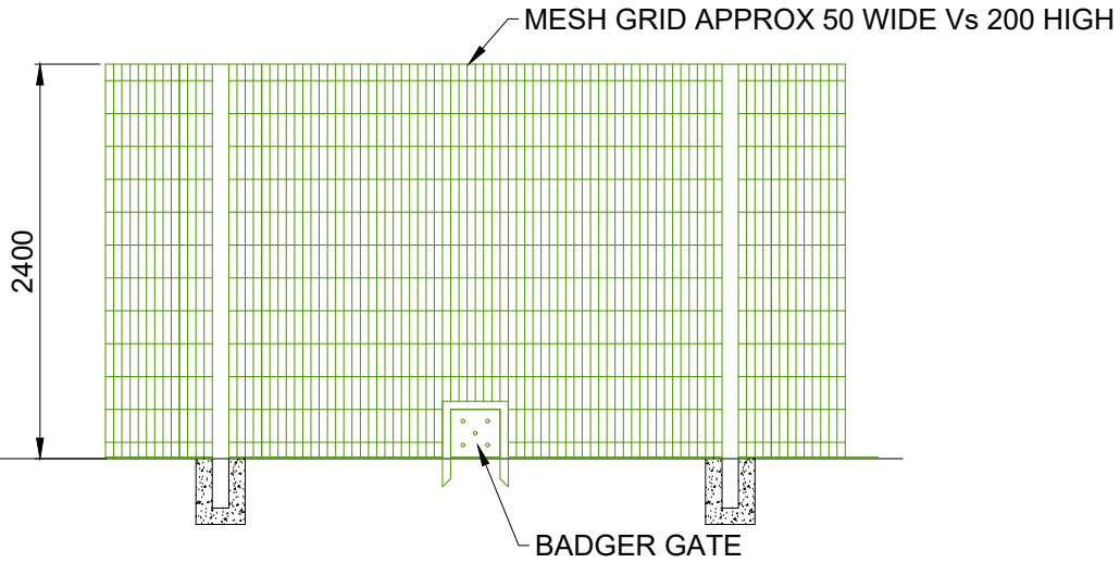
SECURITY FENCE SIDE ELEVATION
