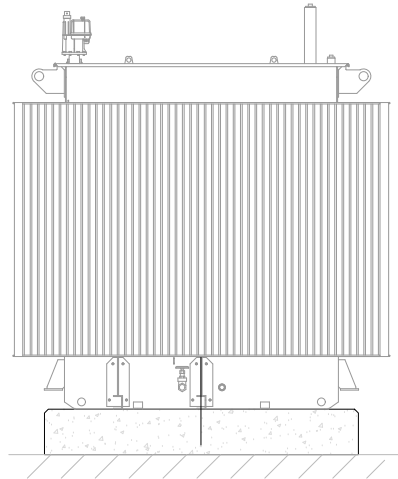
ELEVATION C
