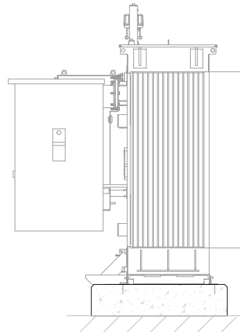
ELEVATION D
